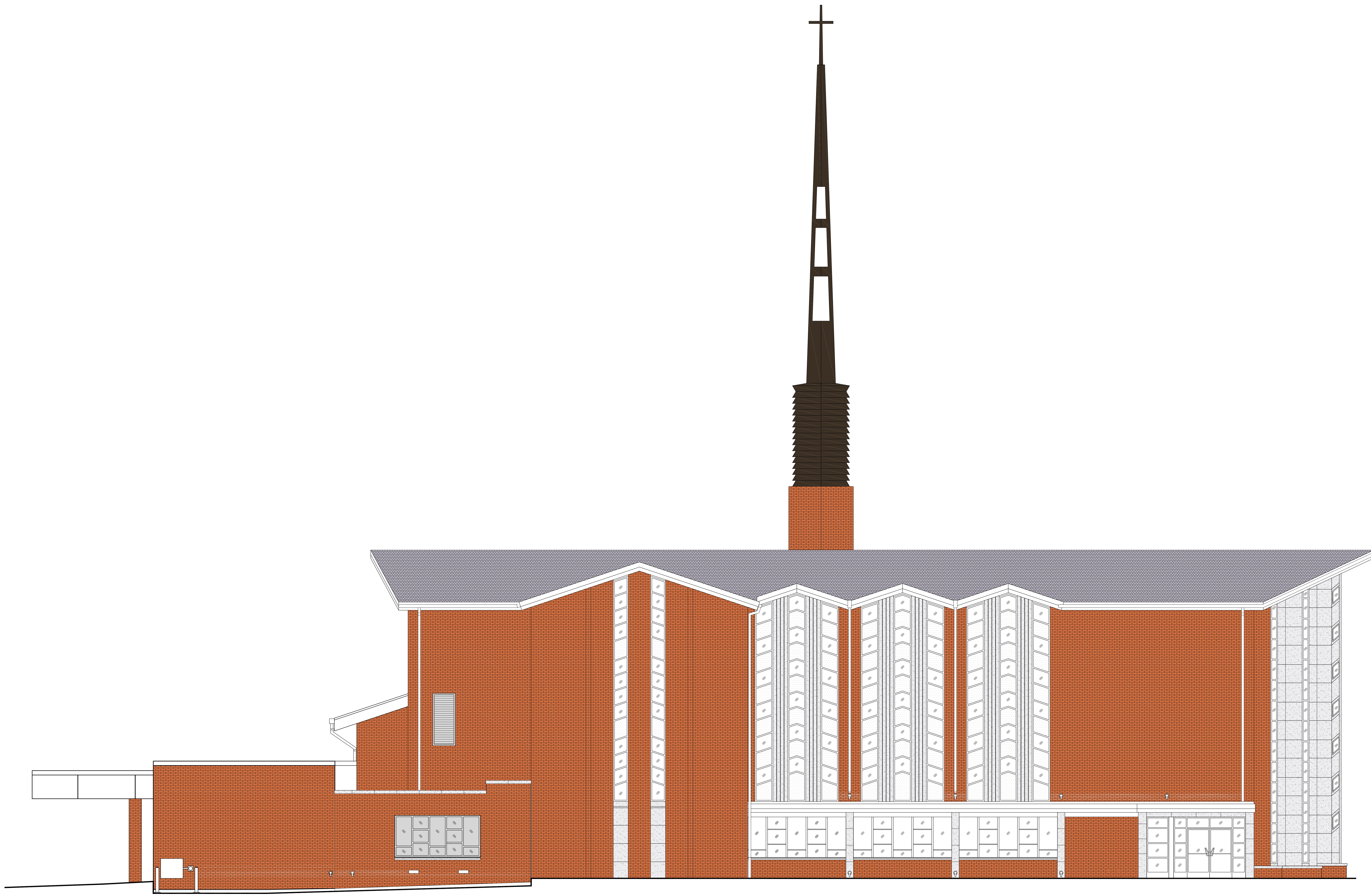
EAST ELEVATION SCALE: 3/16" = 1'-0"
