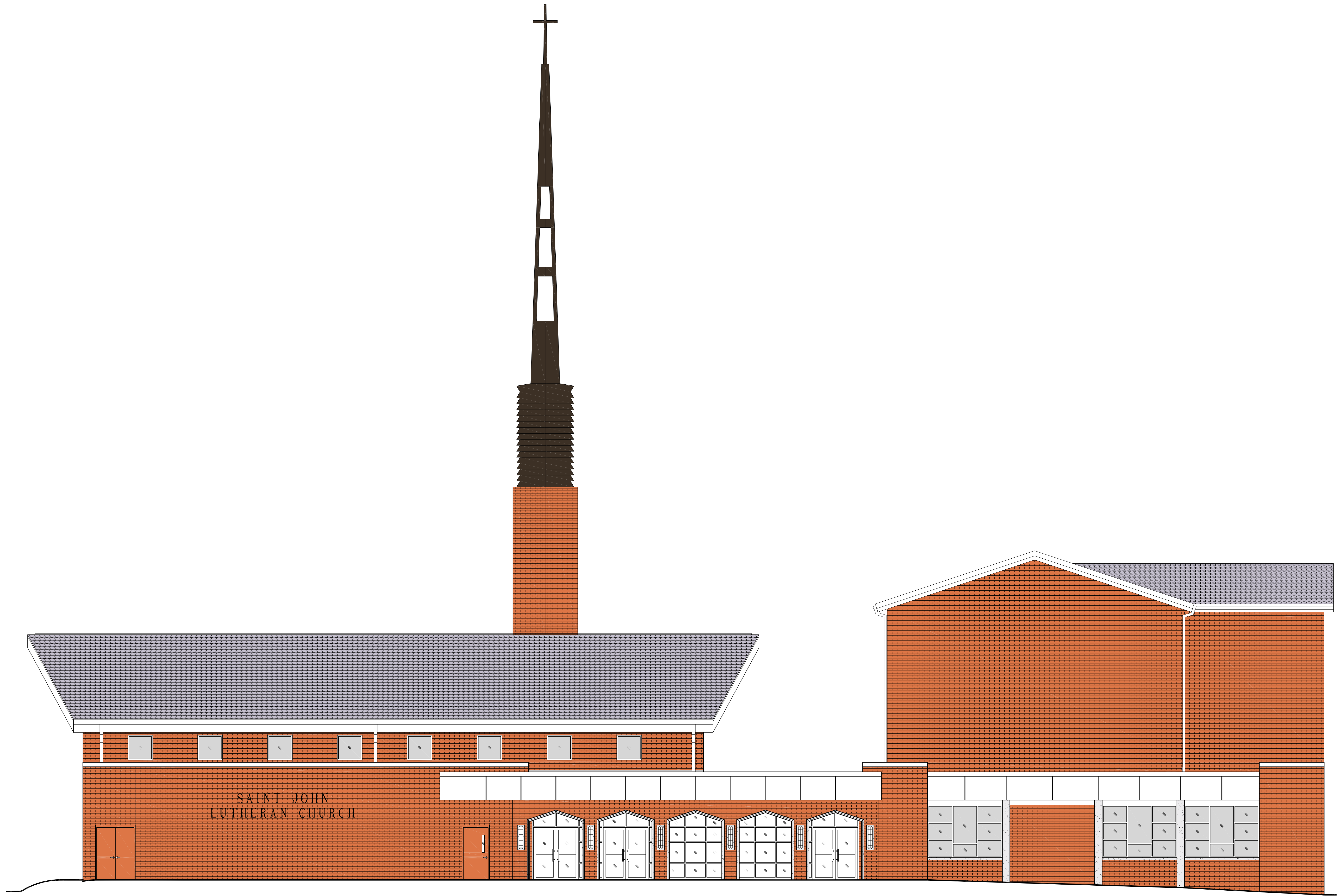
SOUTH ELEVATION SCALE: 3/16" = 1'-0"
